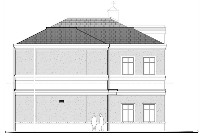
EAST ELEVATION (facing side yard) SCALE: 1 : 100
